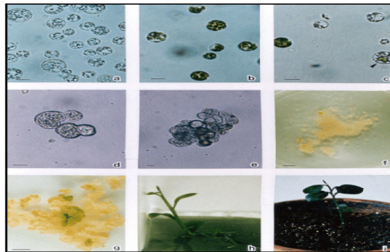
FIG. 1. a. Isolated and purified protoplasts from sweet orange ovule-derived embryogenic callus, in suspension cultures (bar = 10 \mu\text{m} ); b. isolated and purified protoplasts from leaf mesophyll of seedlings germinated in vitro (bar = 10 \mu\text{m} ); c. protoplasts just after the addition of PEG solution. The arrow shows a fusion between an embryogenic suspension and a leaf mesophyll cell derived protoplast (bar = 10 \mu\text{m} ); d. initial cell division, approximately 10 days after protoplast fusion and plating (bar = 10 \mu\text{m} ); e. cell cultures with small colonies (bar = 10 \mu\text{m} ); f. vigorous colonies after transferring to solidified medium (bar = 5 mm); g. somatic embryo induction (bar = 0.5 cm); h. shoots transferred to rooting medium (bar = 0.5 cm); i. regenerated plant, transferred to commercial nutrient mixture in greenhouse (bar = 2.5 cm).
